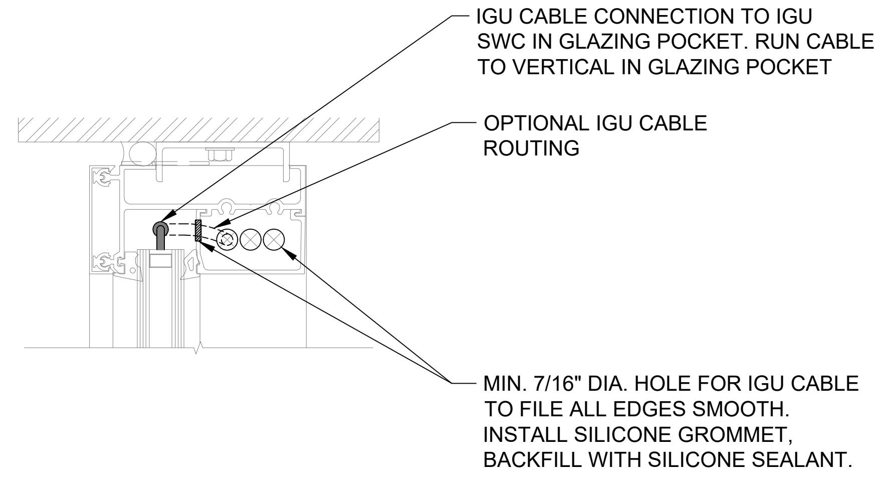
DETAIL 1 HEAD
